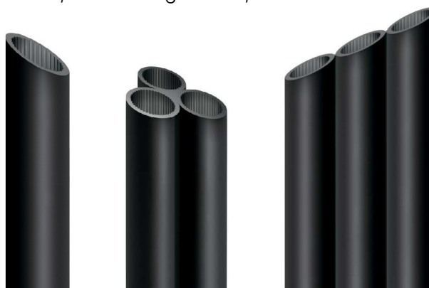
From left to right: single pipe, starlike triple pipe and flat triple pipe in PE, manufactured according to the technical specifications of the main Italian and European managers for optical fibre telecommunication networks.
